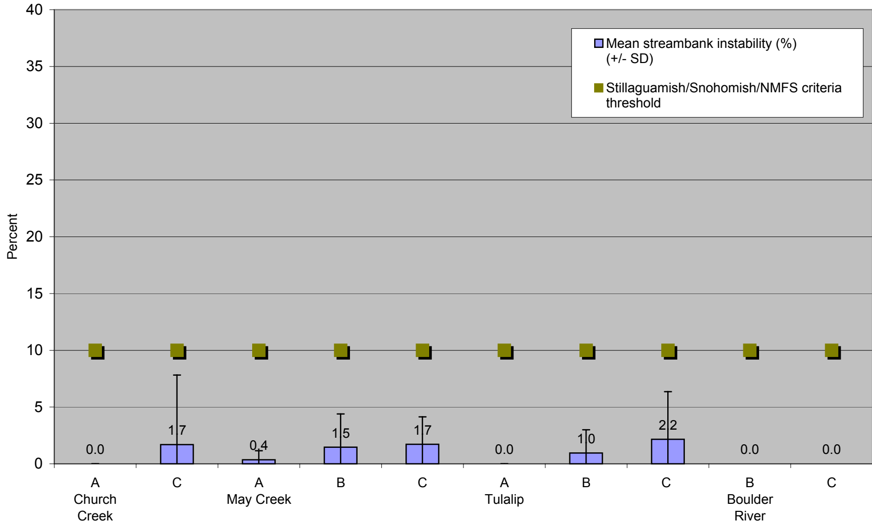
Figure 8. Mean streambank instability (%) by subbasin and Rosgen channel type compared with basin habitat criteria threshold. Values at or below the threshold meet the criteria.
