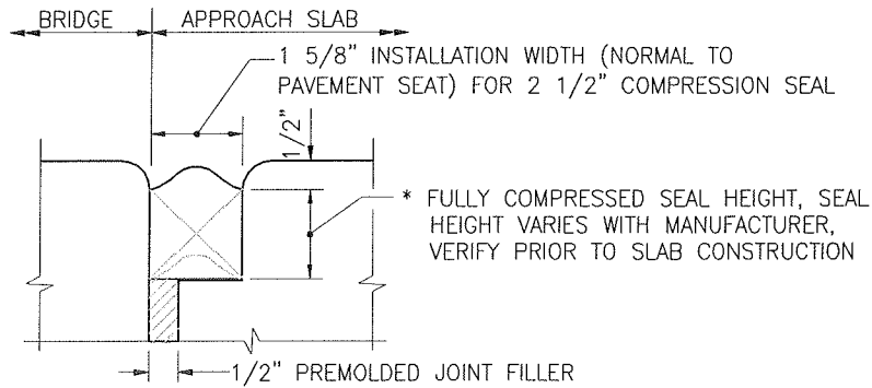
COMPRESSION SEAL DETAIL
