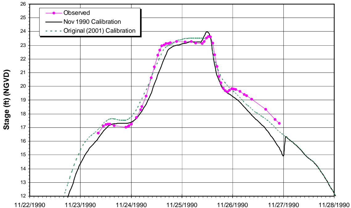
Figure 3. Re-calibration of November 1990 Flood
