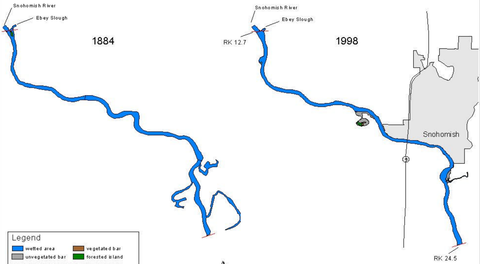
Figure 3-12: Snohomish River channel position in 1884 and 1998 (reach 2)
